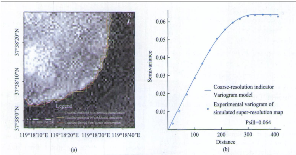
Fig.7 (a) Coastline predicted from the hard classification applied to the original image VS coastline predicted from the geostatistical approach applied to the SIcS image of B in Fig.1; (b) Indicator variogram reproduction for super-resolution realization generated conditional to coarse-resolution spatial structure.
